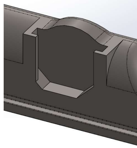
New Design
